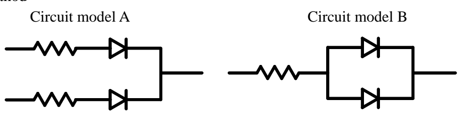
(A)Recommended circuit.
