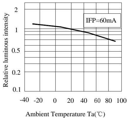
Fig.3 Luminous Intensity vs. Ambient Temperature
