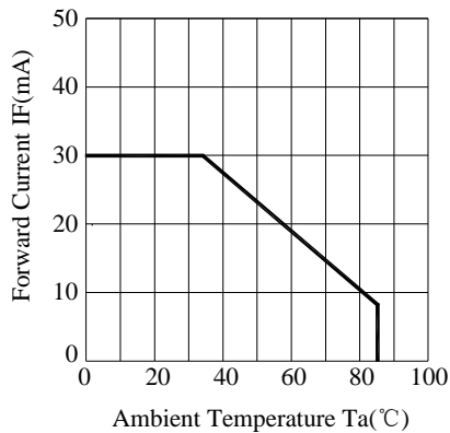
Fig.5 Forward Current Derating Curve
