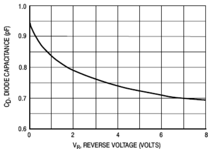
Figure 3. Diode Capacitance
