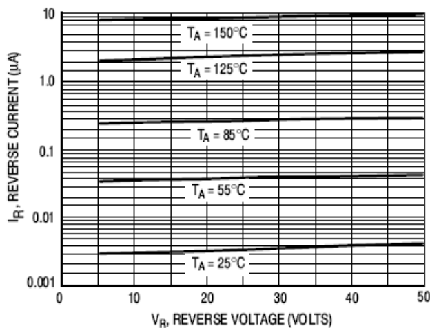
Figure 2. Reverse Current
