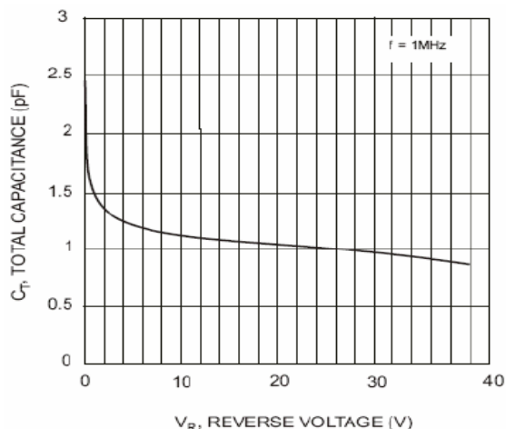
Fig. 3 Typical Total Capacitance vs. Reverse Voltage
