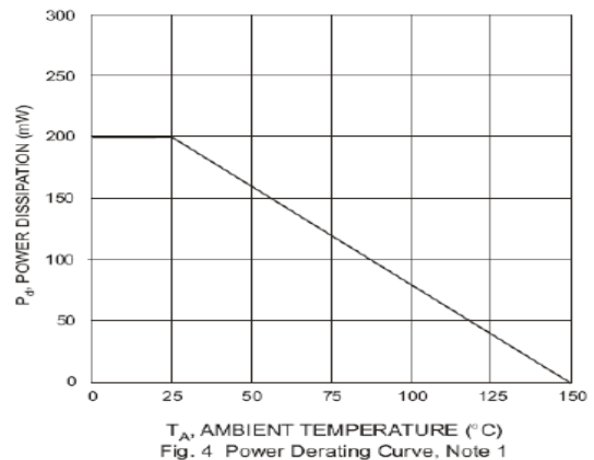
Fig. 4 Power Derating Curve, Note 1
