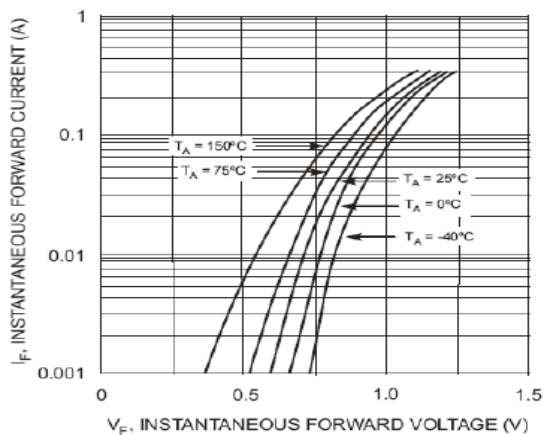
Fig. 1 Forward Characteristics
