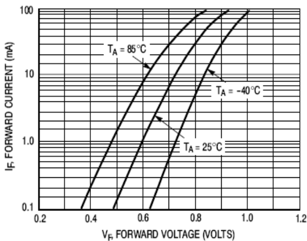
Figure 2. Forward Voltage
