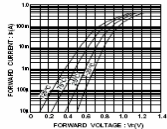
Fig.1 Forward characteristics
