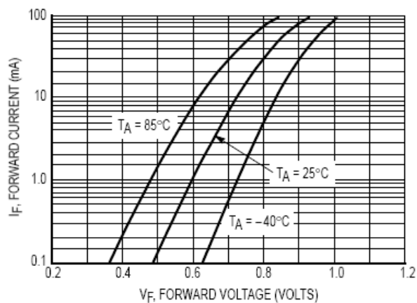
Figure 1. Forward Voltage
