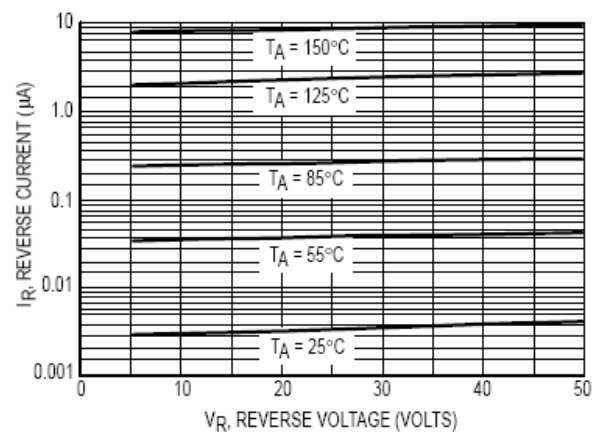
Figure 2. Leakage Current
