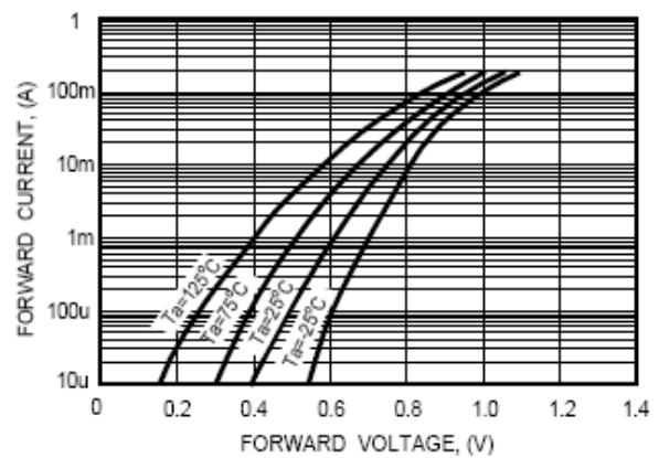
FIG. 2 - FORWARD CHARACTERISTICS
