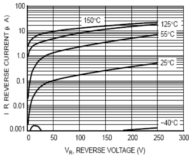
Figure 3. Leakage Current
