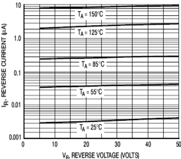
Figure 3. Leakage Current
