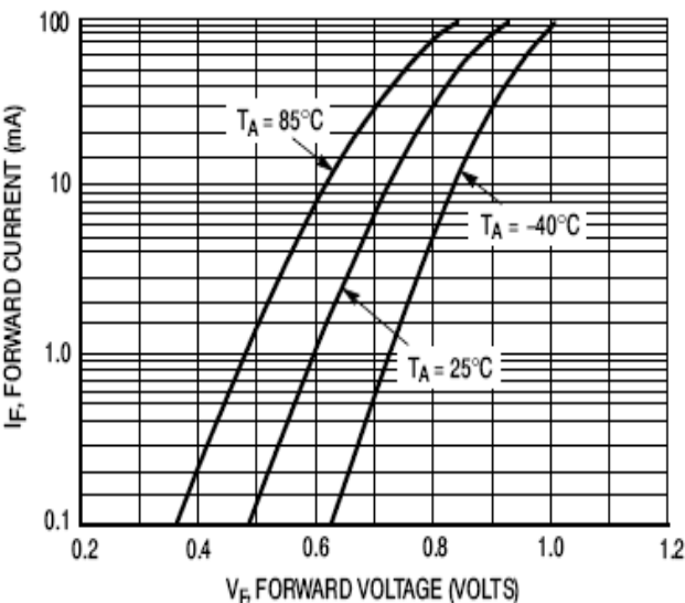
Figure 2. Forward Voltage
