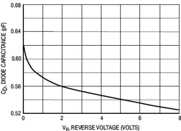
Figure 4. Capacitance
