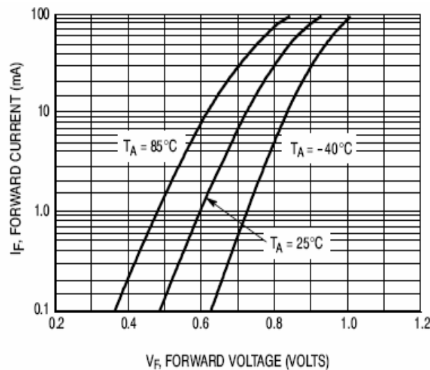
Figure 1. Forward Voltage
