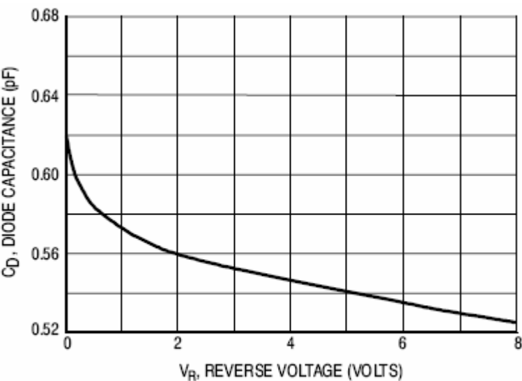
Figure 3. Capacitance
