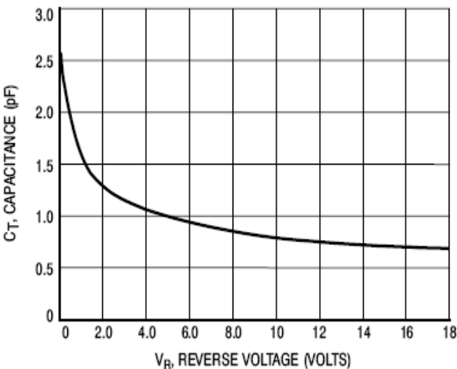
Figure 4. Typical Capacitance
