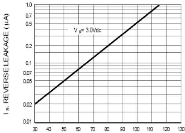
T_A , AMBIENT TEMPERATURE (°C) Figure 1. Reverse Leakage
