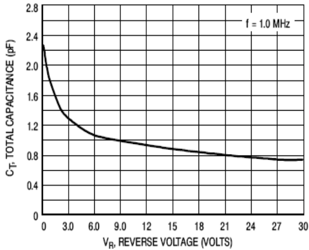
Figure 1. Total Capacitance
