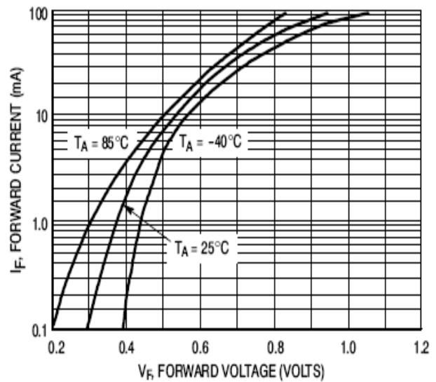
Figure 4. Forward Voltage
