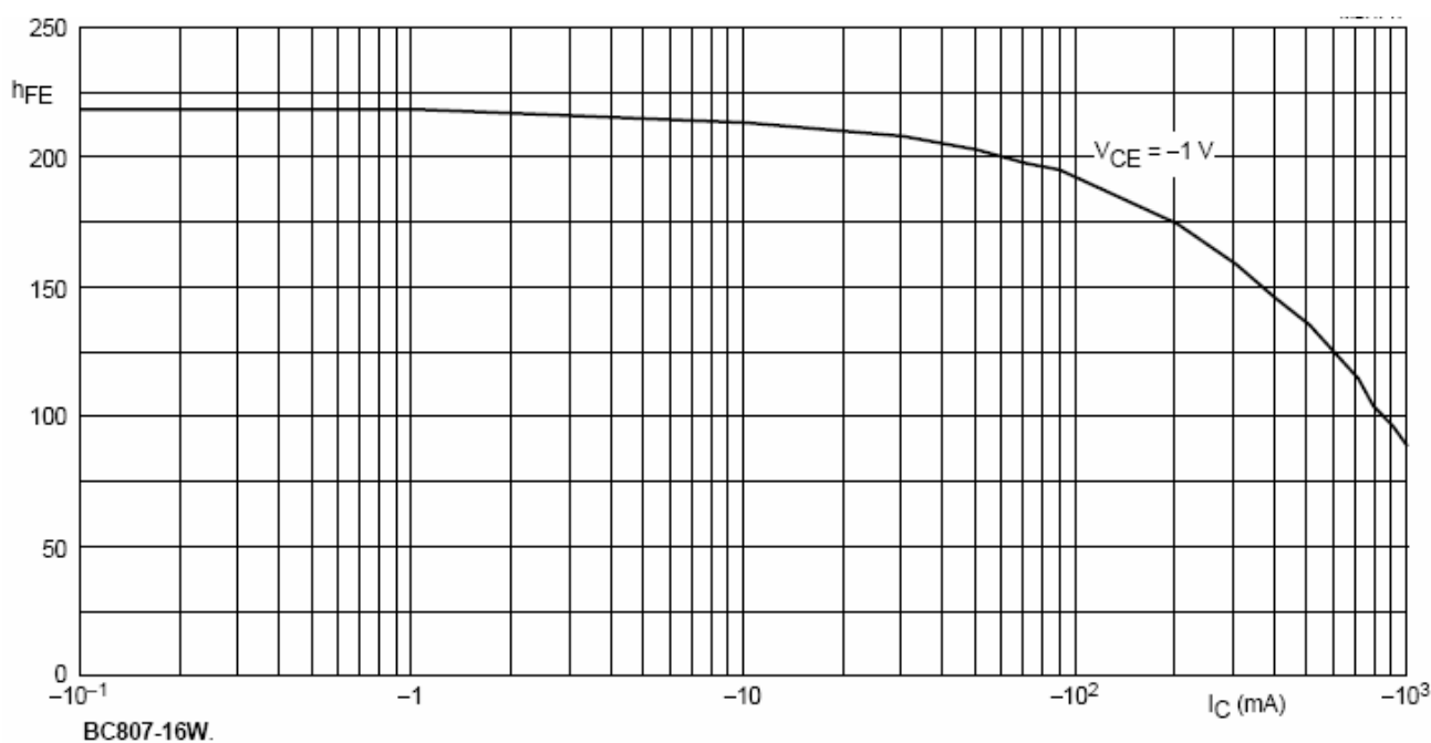
Fig.1 DC current gain; typical values.
