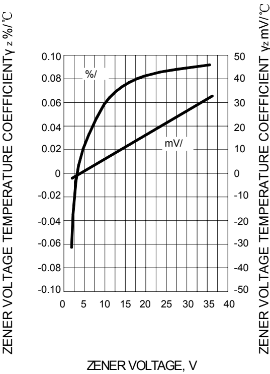
FIG.2 – TEMPERATURE COEFFICIENT
