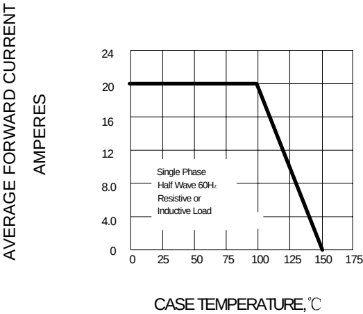
FIG.4-FORWARD DERATING CURVE
