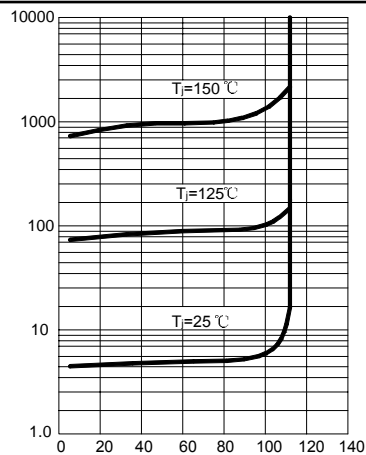
FIG.4 – TYPICAL REVERSE CHARACTERISTICS
