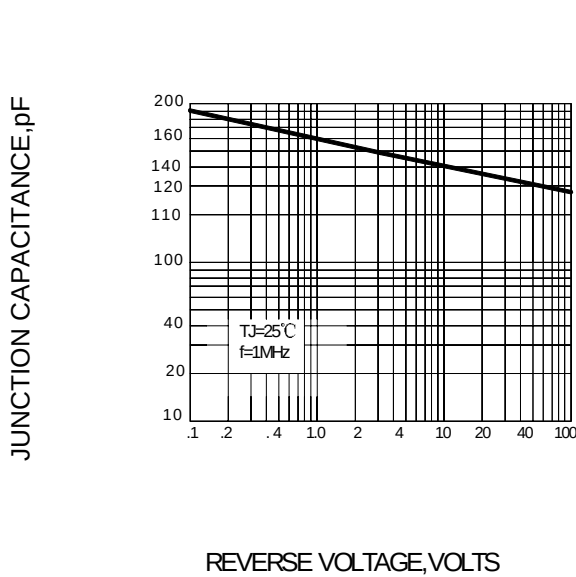
FIG.5 – PEAK JUNCTION CAPACITANCE
