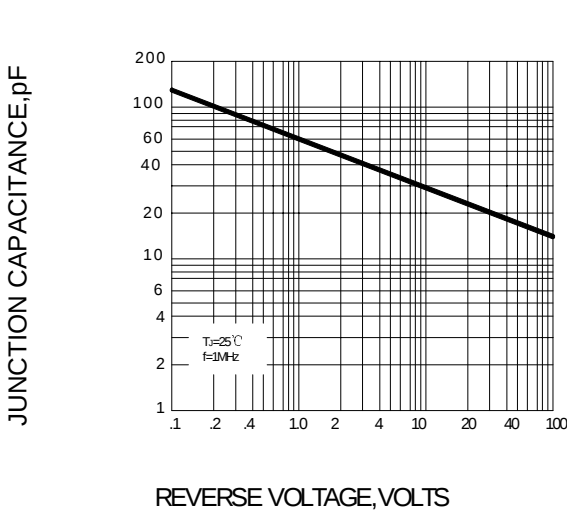
FIG.4-TYPICAL JUNCTION CAPACITANCE
