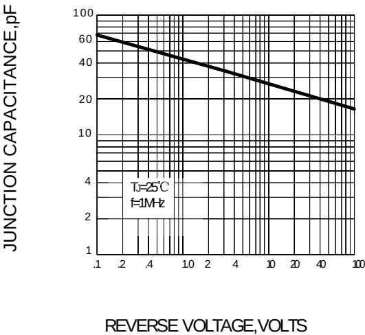
FIG.4-TYPICAL JUNCTION CAPACITANCE
