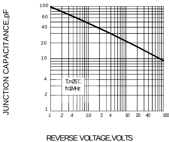
FIG.4-TYPICAL JUNCTION CAPACITANCE
