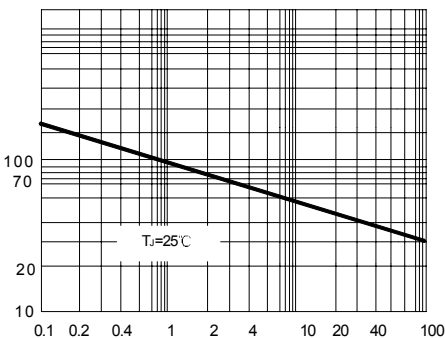
FIG.6–TYPICAL JUNCTION CAPACITANCE
