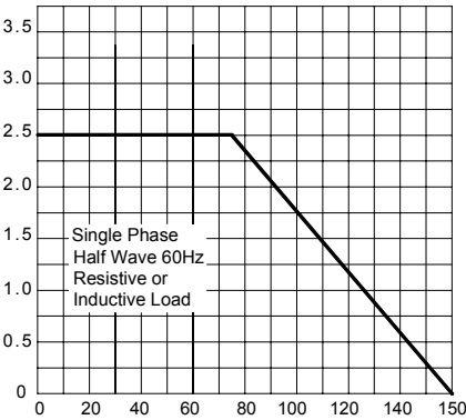
FIG.3 –FORWARD DERATING CURVE
