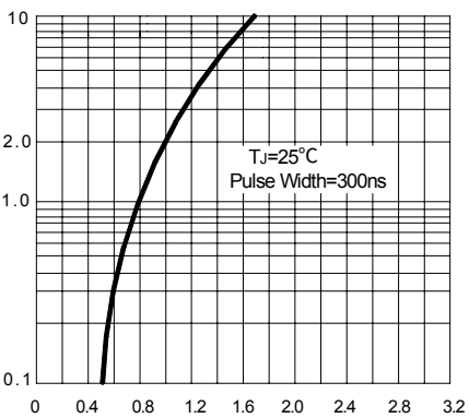
FIG.4–TYPICAL FORWARD CHARACTERISTIC
