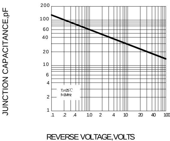
FIG.4-TYPICAL JUNCTION CAPACITANCE
