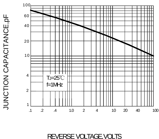
FIG.4- PEAK JUNCTION CAPACITANCE
