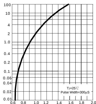
FIG.3 – TYPICAL FORWARD CHARACTERISTIC
