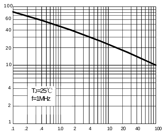
FIG.4- PEAK JUNCTION CAPACITANCE
