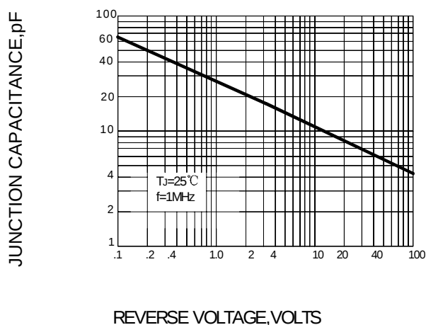
FIG.4–TYPICAL JUNCTION CAPACITANCE
