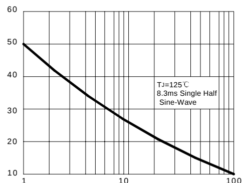
FIG.3 – PEAK FORWARD SURGE CURRENT
