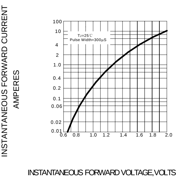
FIG.4-TYPICAL FORWARD CHARACTERISTIC
