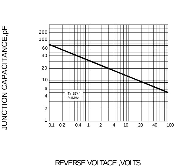
FIG.5-TYPICAL JUNCTION CAPACITANCE
