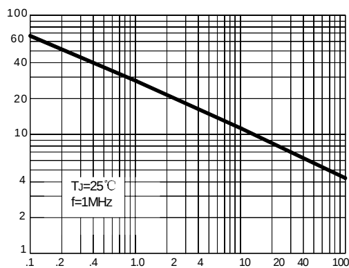
FIG.4-TYPICAL JUNCTION CAPACITANCE
