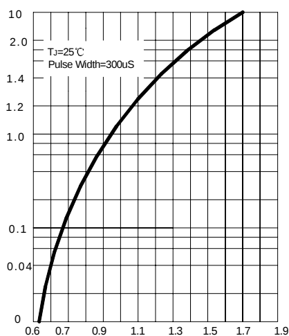
FIG.2 – TYPICAL FORWARD CHARACTERISTIC
