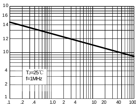
FIG.4-TYPICAL JUNCTION CAPACITANCE
