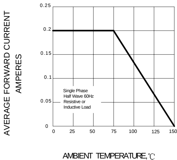
FIG.2 – TYPICAL FORWARD DERATING CURVE
