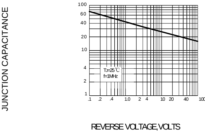
FIG.5-TYPICAL JUNCTION CAPTACNCE
