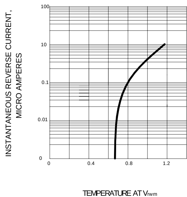
FIG.3-- TYPICAL REVERSE CHARACTERISTIC
