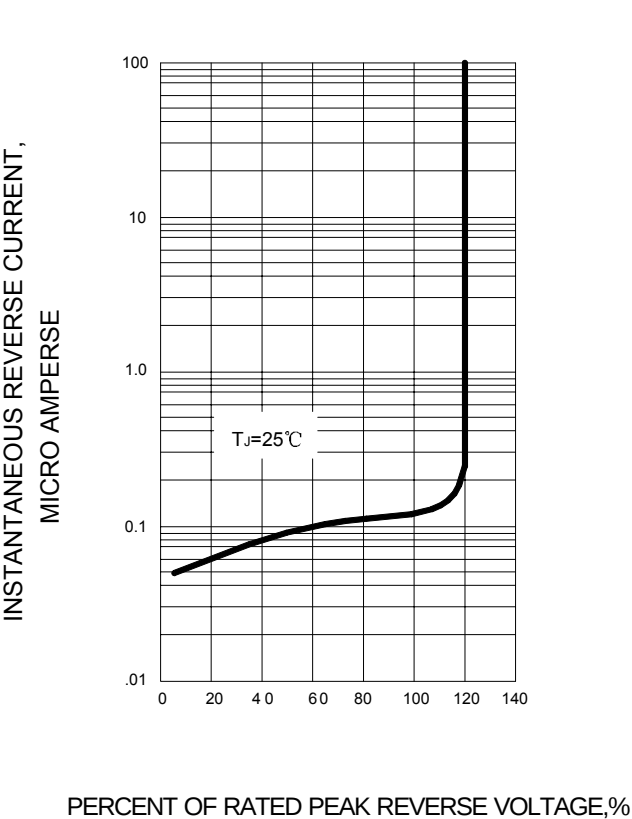
FIG.4 – TYPICAL REVERSE CHARACTERISTIC
