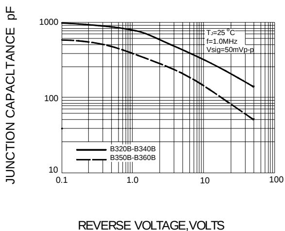
FIG.5-TYPICAL JUNCTION CAPACITANCE
