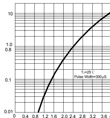
FIG.5 - TYPICAL FORWARD CHARACTERISTIC
