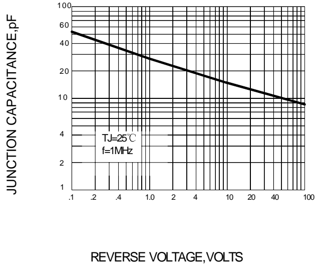
FIG.2 – JUNCTION CHARACTERISTICS
