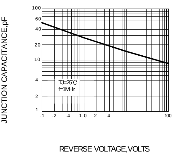
FIG.2 -- JUNCTION CHARACTERISTICS
