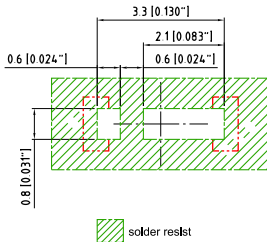
solder resist
