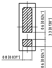
solder resist
