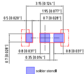
solder stencil
