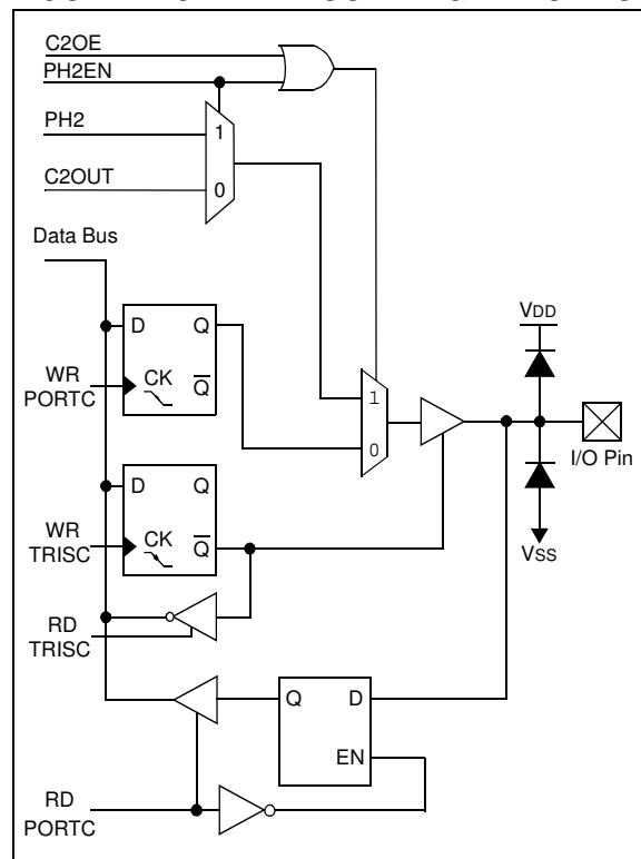
FIGURE 4-13: BLOCK DIAGRAM OF RC4
