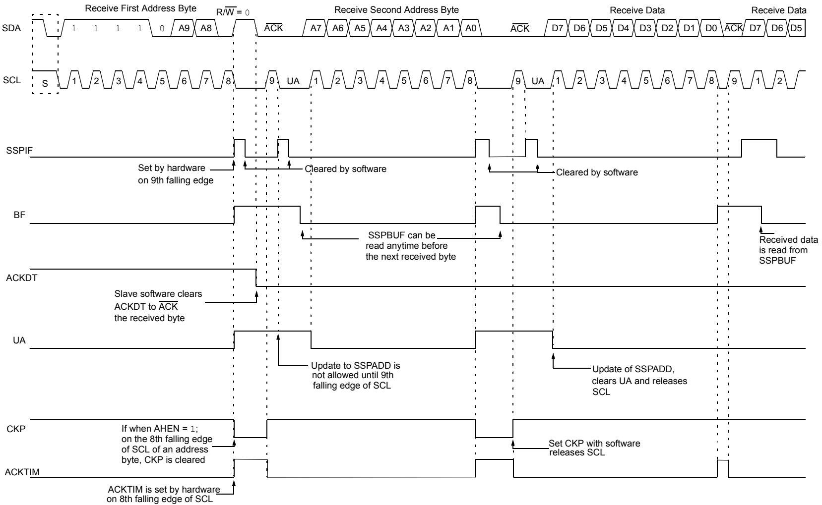
FIGURE 26-21: I 2 C SLAVE, 10-BIT ADDRESS, RECEPTION (SEN = 0, AHEN = 1, DHEN = 0)
