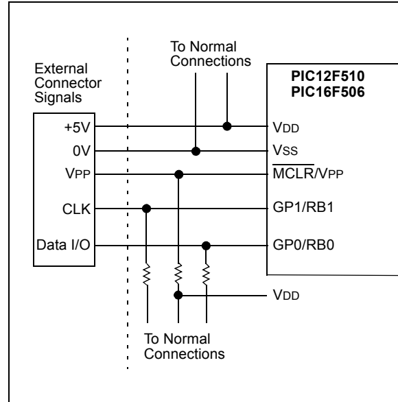
FIGURE 10-15: TYPICAL IN-CIRCUIT SERIAL PROGRAMMING CONNECTION
