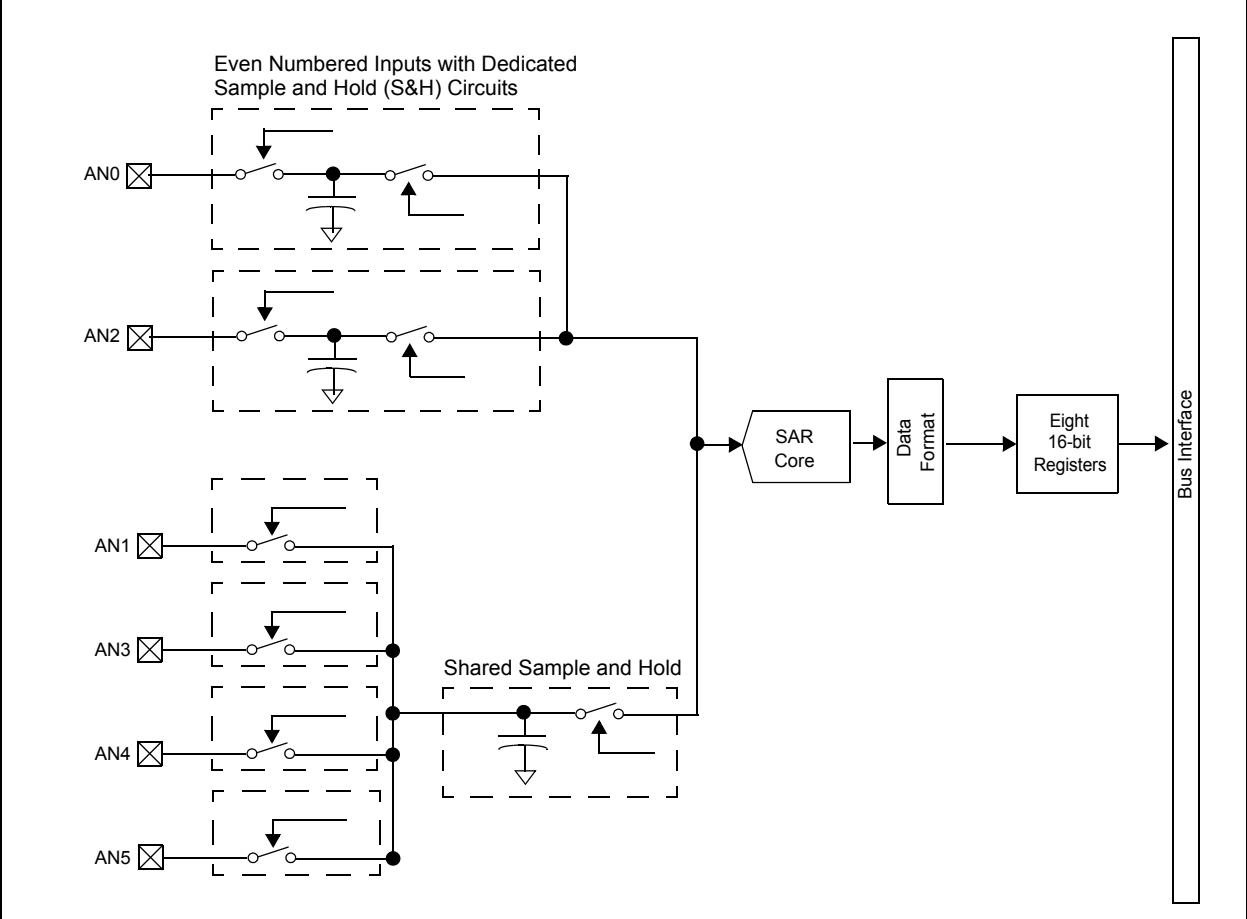
FIGURE 19-3: ADC BLOCK DIAGRAM FOR dsPIC33FJ06GS102A DEVICE
