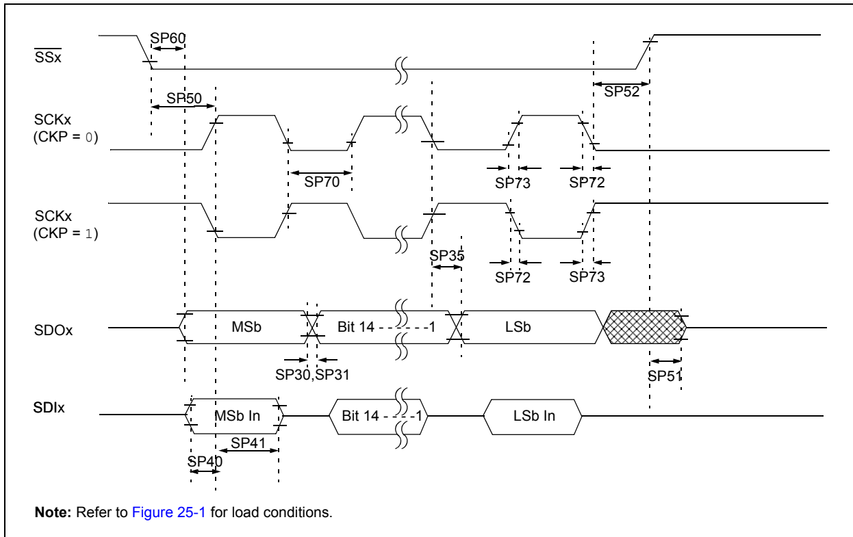
FIGURE 25-15: SPIx SLAVE MODE (FULL-DUPLEX, CKE = 1, CKP = 0, SMP = 0) TIMING CHARACTERISTICS
