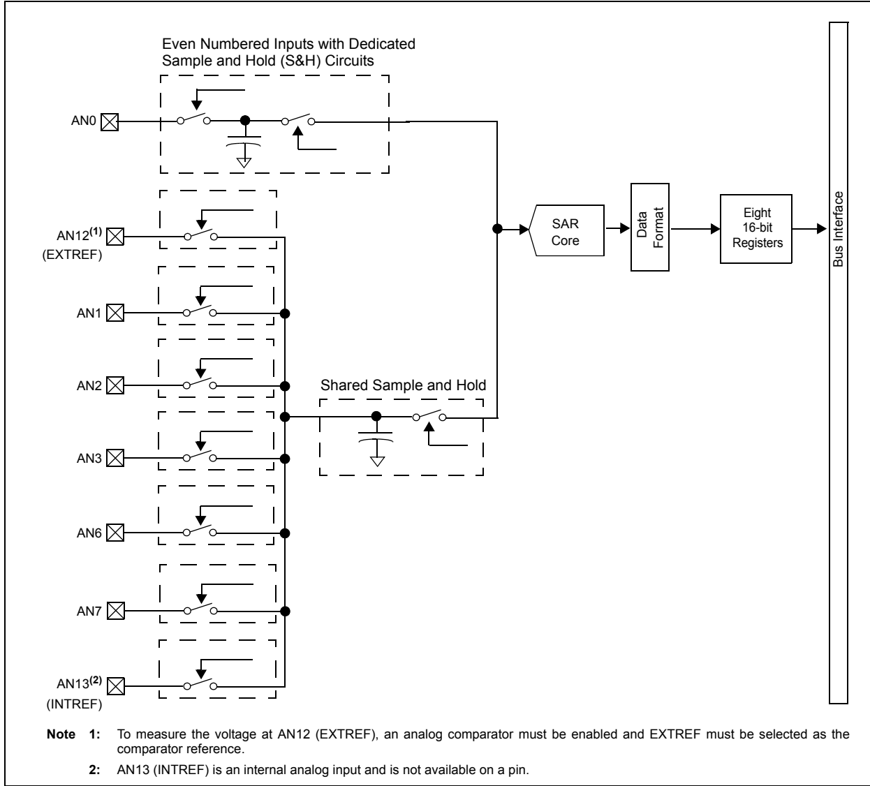
FIGURE 19-1: ADC BLOCK DIAGRAM FOR THE dsPIC33FJ06GS001 DEVICE
