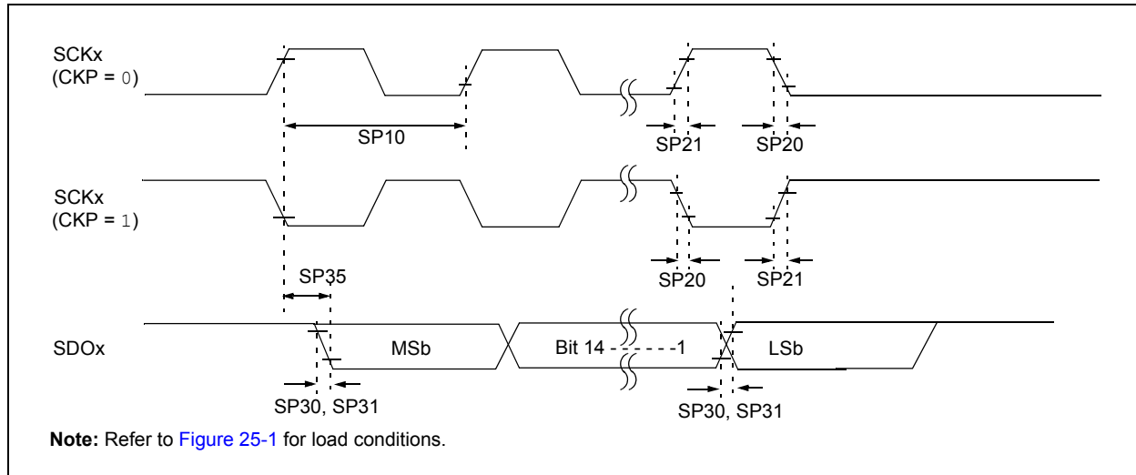
FIGURE 25-11: SPIx MASTER MODE (HALF-DUPLEX, TRANSMIT ONLY CKE = 0) TIMING CHARACTERISTICS
