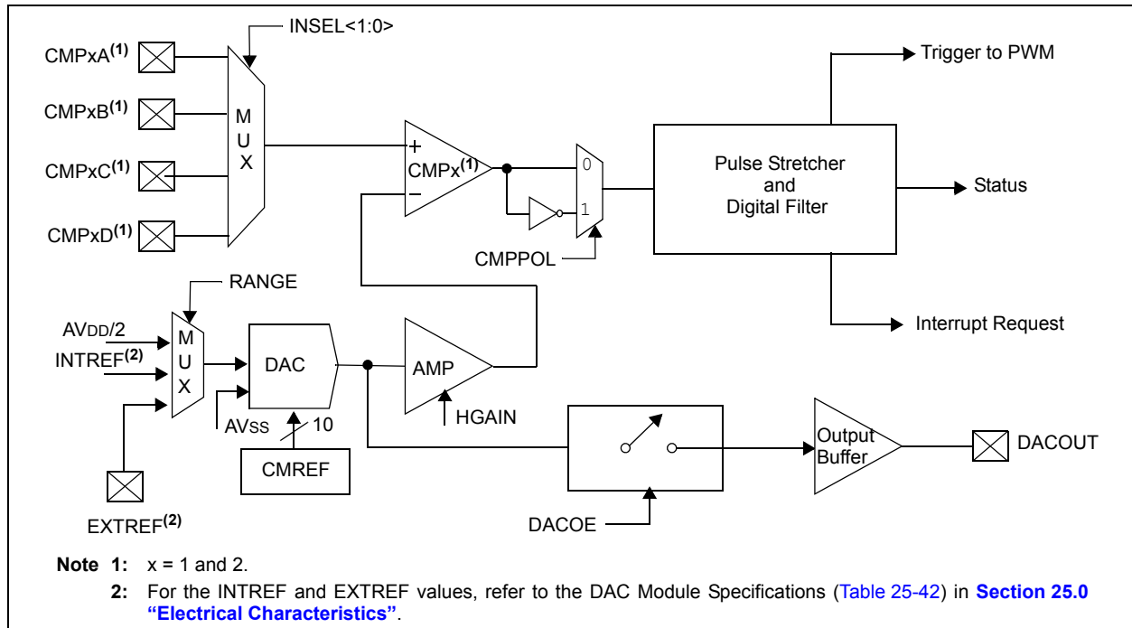
FIGURE 20-1: HIGH-SPEED COMPARATOR MODULE BLOCK DIAGRAM
