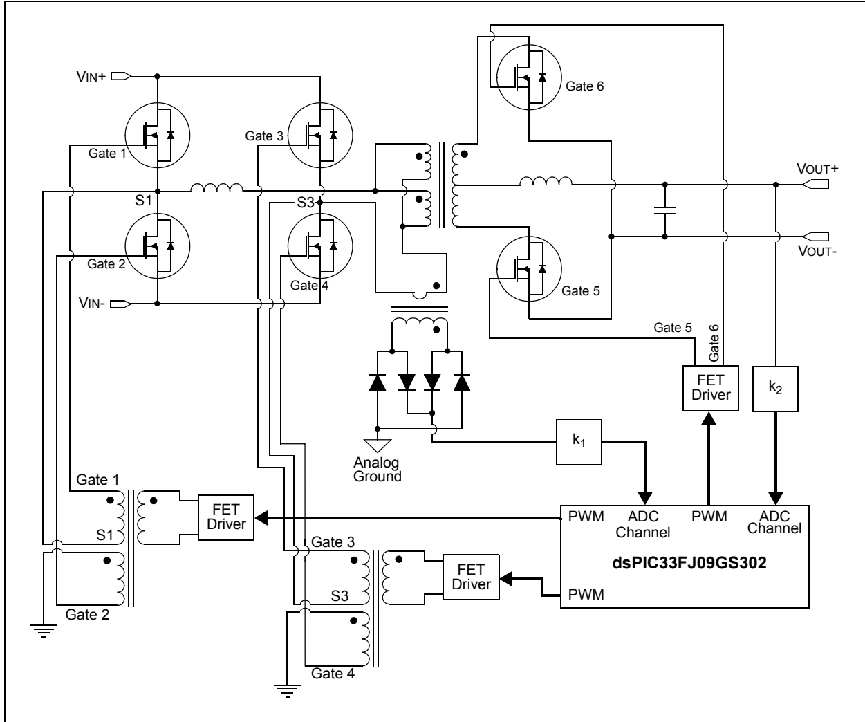
FIGURE 2-8: PHASE-SHIFTED FULL-BRIDGE CONVERTER
