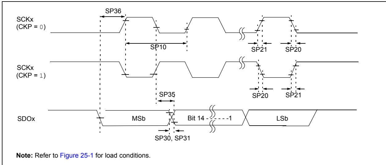
FIGURE 25-12: SPIx MASTER MODE (HALF-DUPLEX, TRANSMIT ONLY) TIMING CHARACTERISTICS
