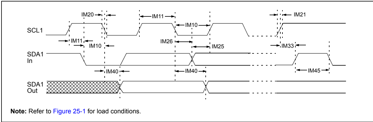
FIGURE 25-20: I2C1 BUS DATA TIMING CHARACTERISTICS (MASTER MODE)
