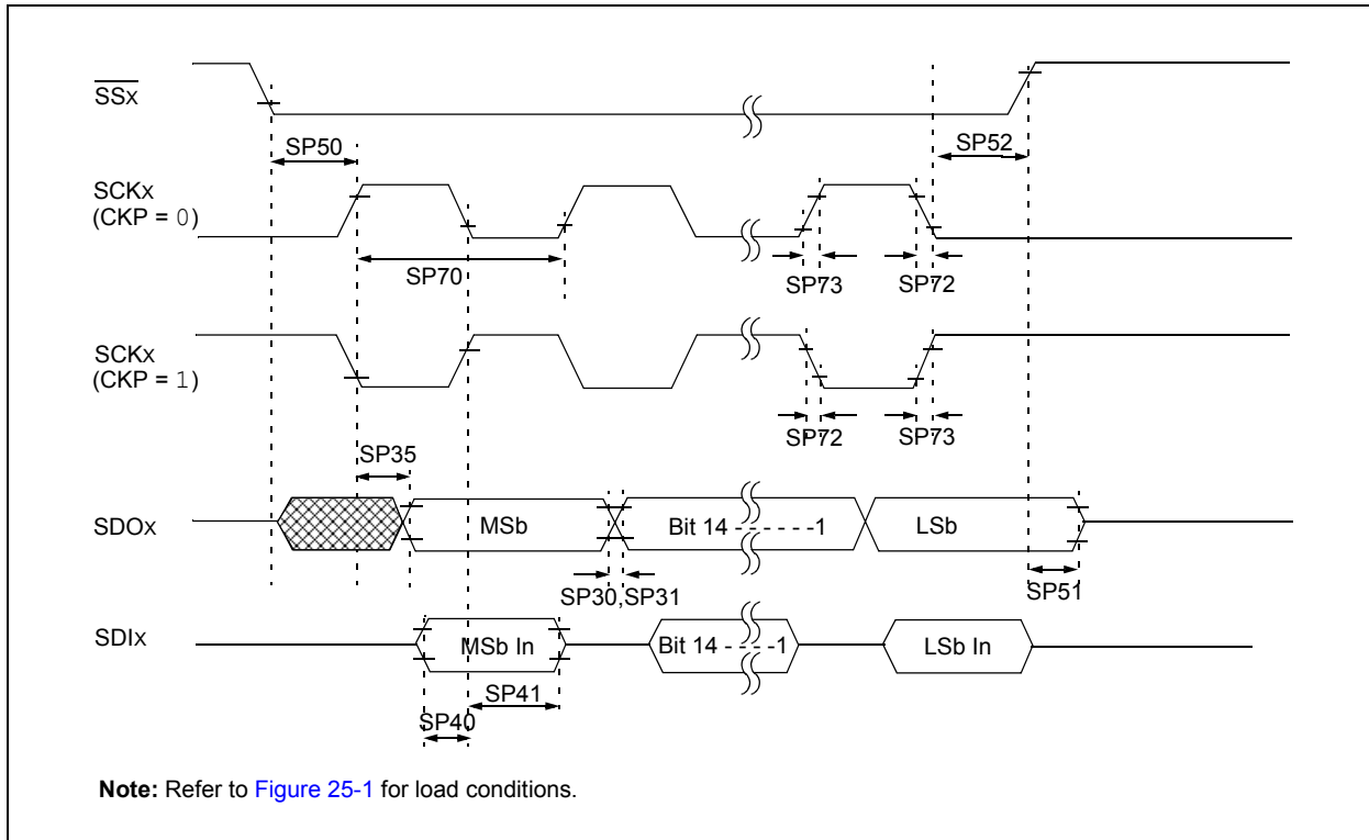
FIGURE 25-17: SPIx SLAVE MODE (FULL-DUPLEX CKE = 0, CKP = 1, SMP = 0) TIMING CHARACTERISTICS
