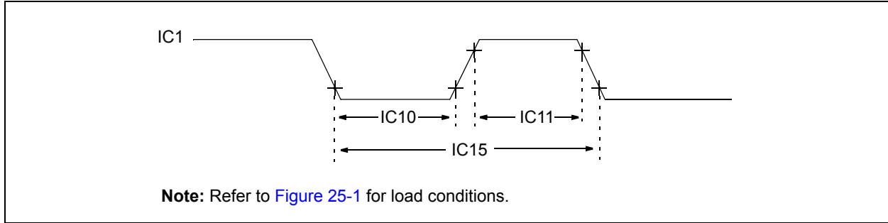
FIGURE 25-6: INPUT CAPTURE (CAP1) TIMING CHARACTERISTICS
