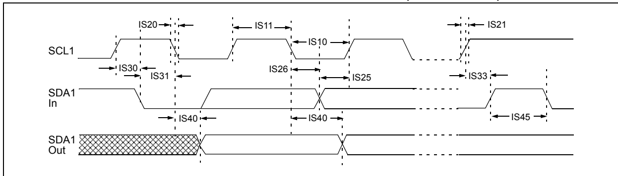
FIGURE 25-22: I2C1 BUS DATA TIMING CHARACTERISTICS (SLAVE MODE)
