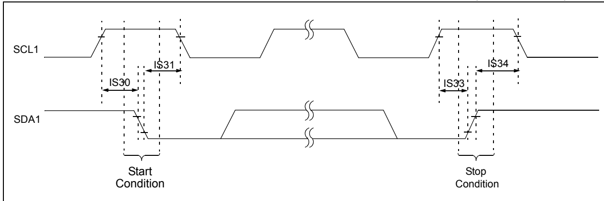
FIGURE 25-21: I2C1 BUS START/STOP BITS TIMING CHARACTERISTICS (SLAVE MODE)
