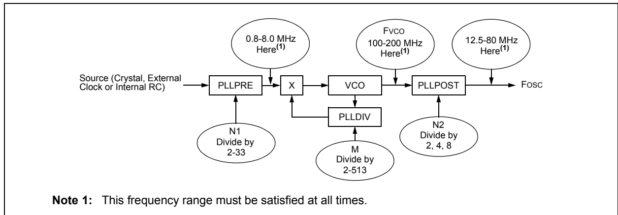
FIGURE 8-2: dsPIC33FJ06GS001/101A/102A/202A and dsPIC33FJ09GS302 PLL BLOCK DIAGRAM
