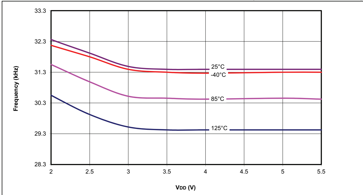
FIGURE 26-25: PIC18F1XK22 TYPICAL LF-INTOSC FREQUENCY (MAX./MIN. = 31.25 kHz \pm 15%)
