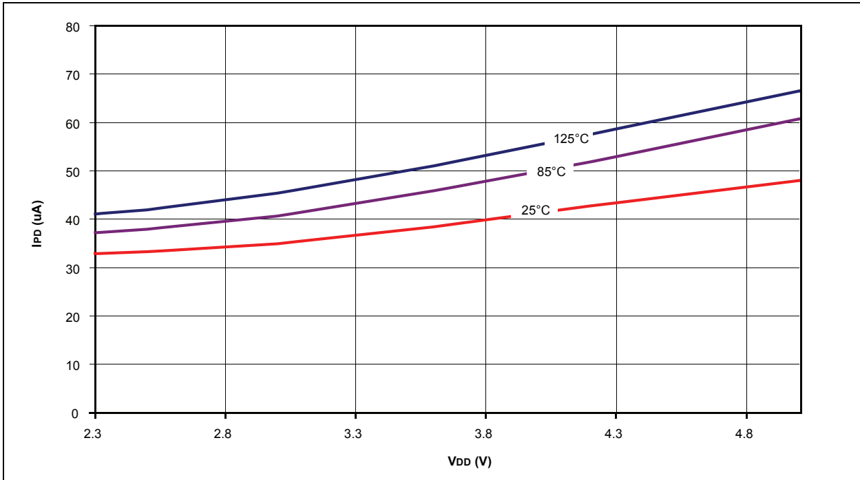
FIGURE 26-14: PIC18F1XK22 TYPICAL I PD FOR COMPARATOR VOLTAGE REFERENCE
