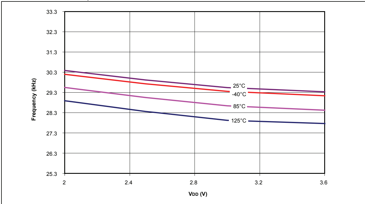
FIGURE 26-27: PIC18LF1XK22 TYPICAL LF-INTOSC FREQUENCY (MAX./MIN. = 31.25 kHz \pm 15%)
