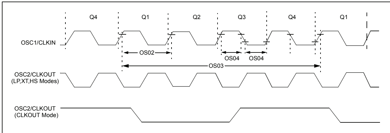
FIGURE 25-8: CLOCK TIMING
