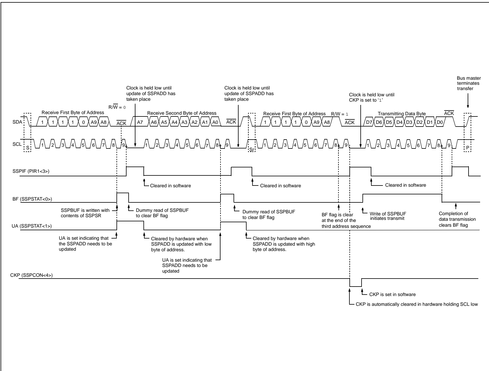
FIGURE 10-11: I 2 C™ SLAVE MODE TIMING (TRANSMISSION, 10-BIT ADDRESS)
