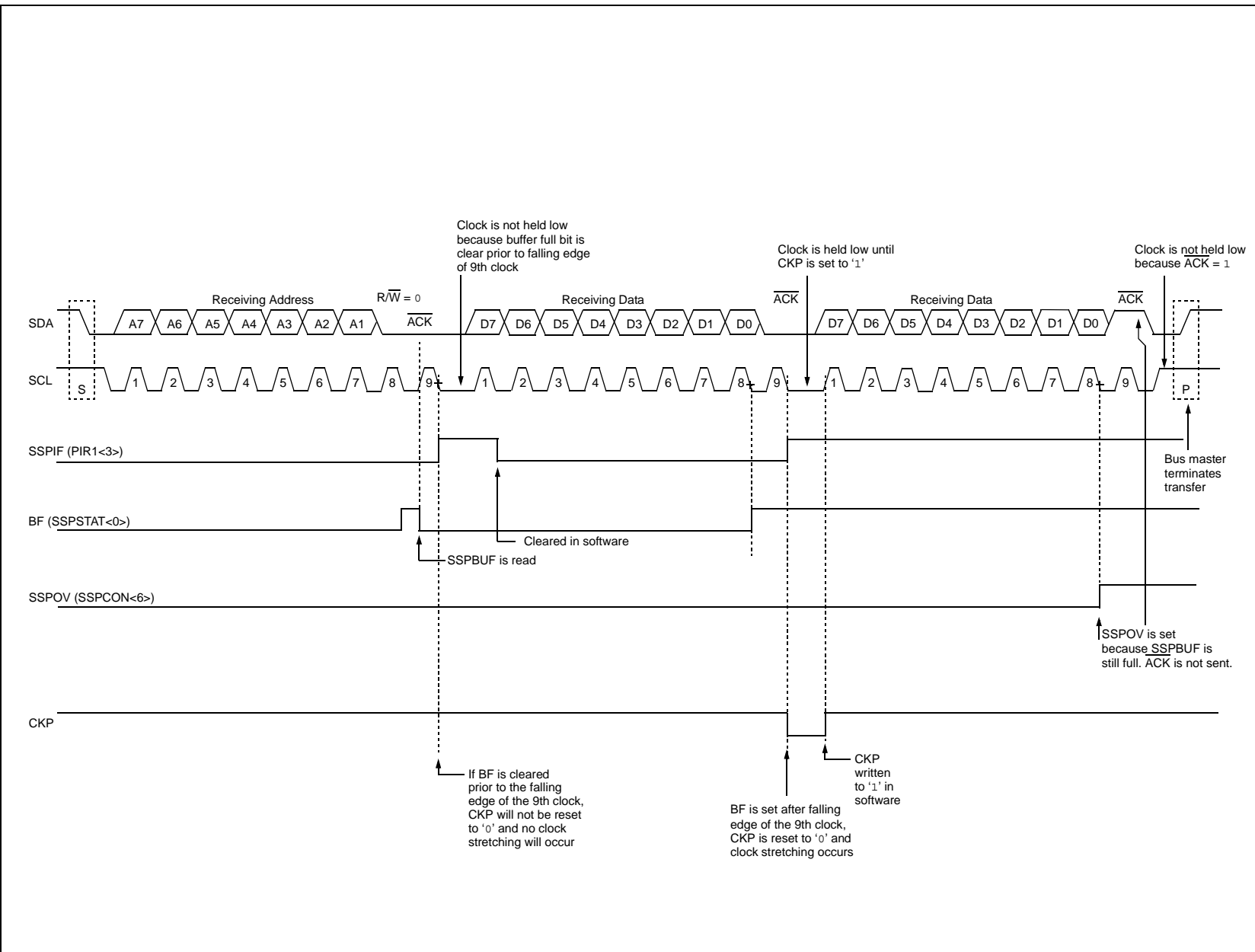
FIGURE 10-13: I 2 C™ SLAVE MODE TIMING WITH SEN = 1 (RECEPTION, 7-BIT ADDRESS)
