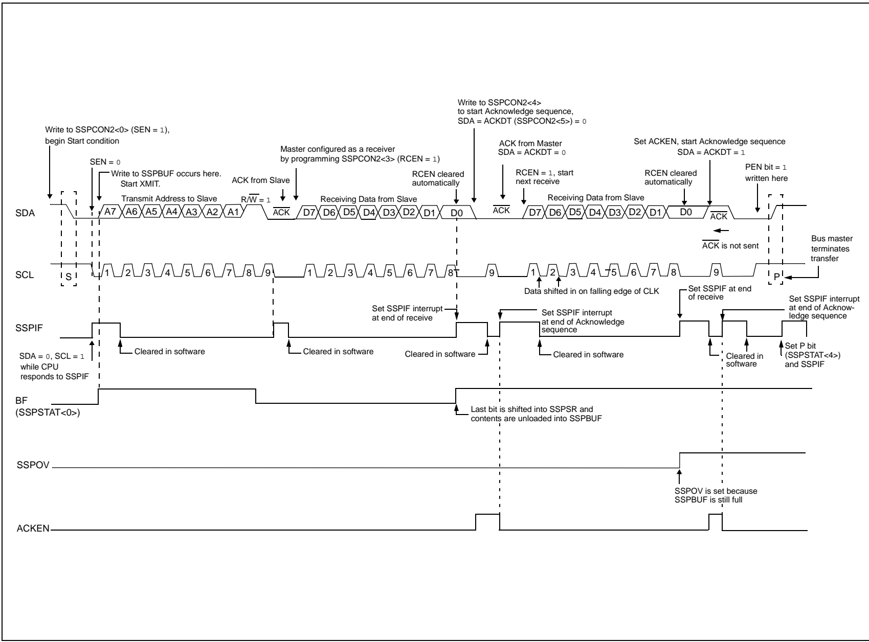
FIGURE 10-22: I 2 C™ MASTER MODE WAVEFORM (RECEPTION, 7-BIT ADDRESS)
