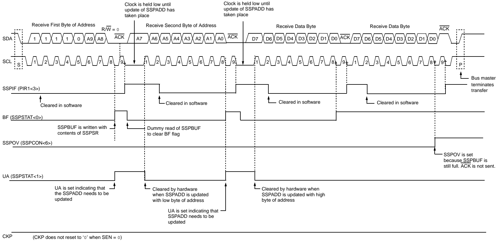
FIGURE 10-10: I 2 C™ SLAVE MODE TIMING WITH SEN = 0 (RECEPTION, 10-BIT ADDRESS)
