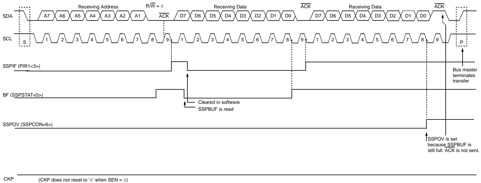
FIGURE 10-8: I 2 C™ SLAVE MODE TIMING WITH SEN = 0 (RECEPTION, 7-BIT ADDRESS)
