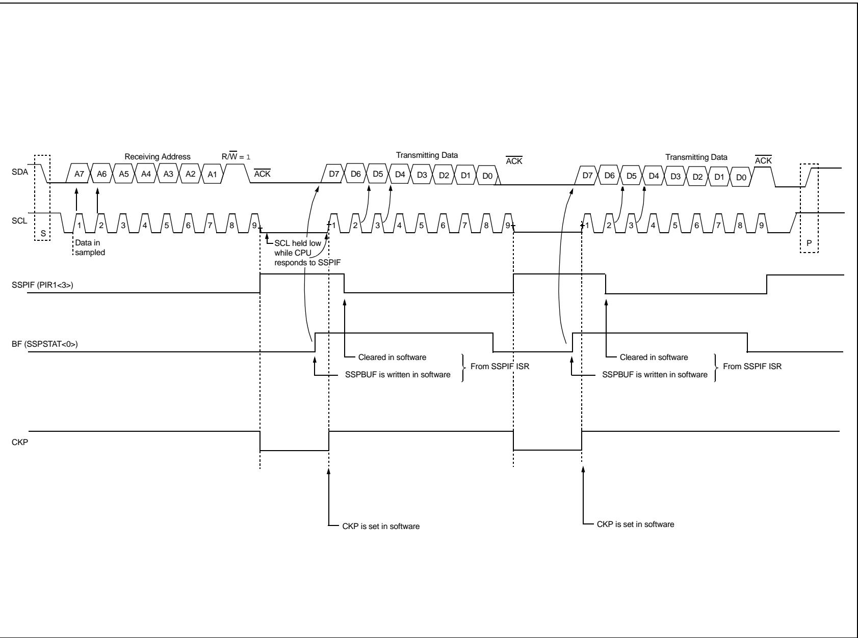
FIGURE 10-9: I 2 C™ SLAVE MODE TIMING (TRANSMISSION, 7-BIT ADDRESS)
