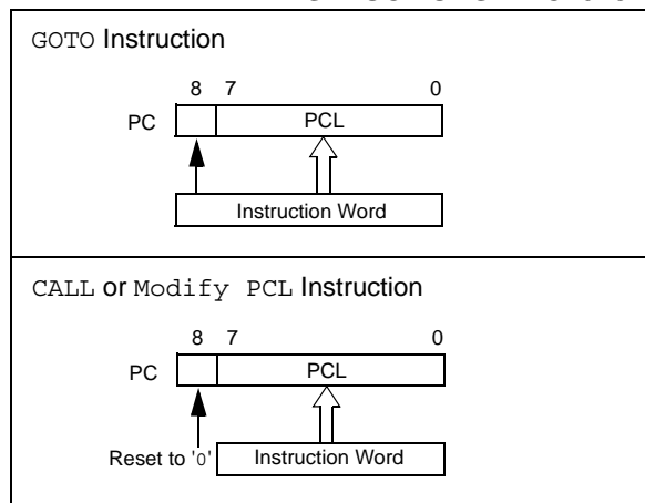
FIGURE 3-6: LOADING OF PC BRANCH INSTRUCTIONS – PIC16F54
