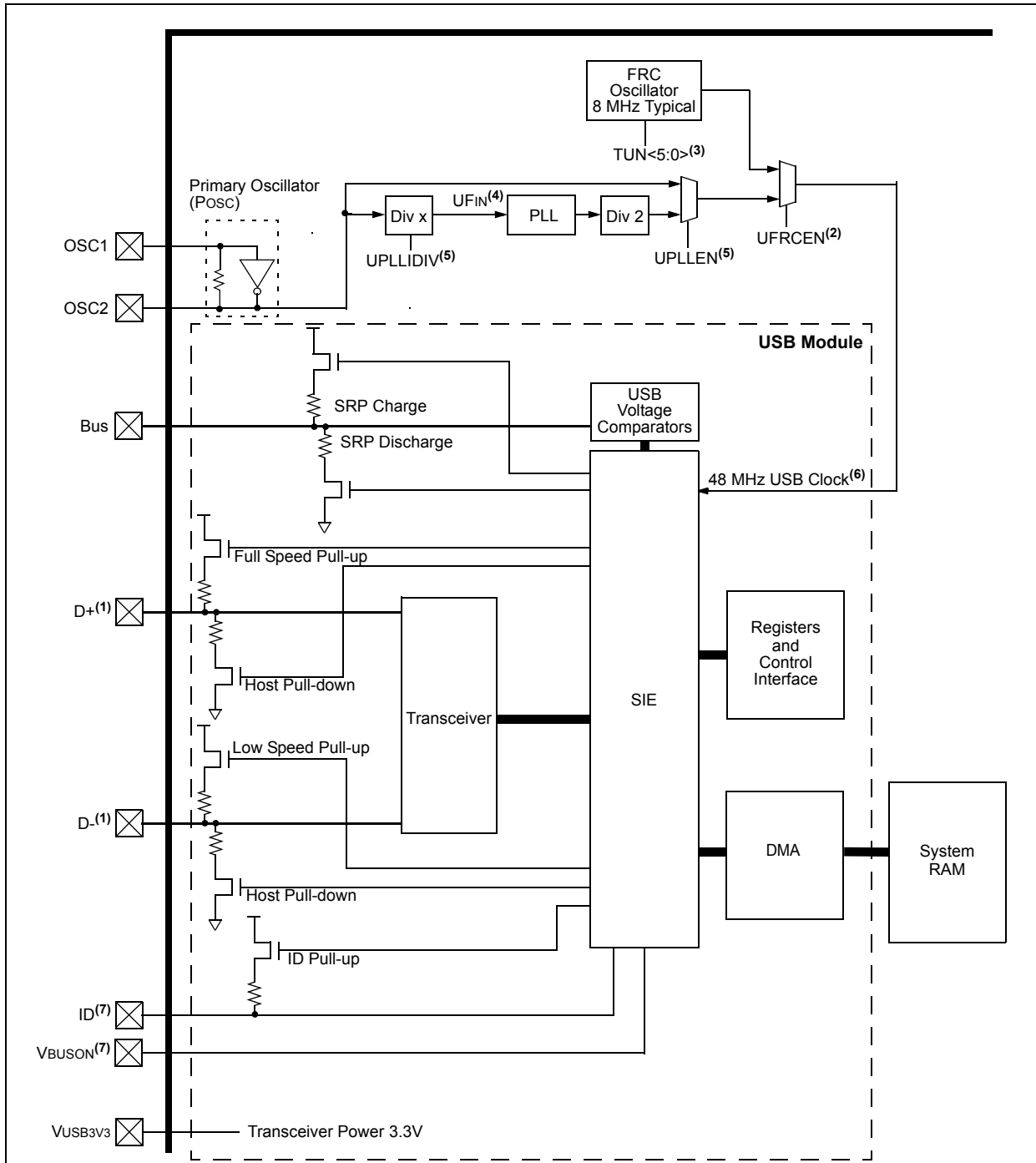
FIGURE 10-1: PIC32MX1XX/2XX FAMILY USB INTERFACE DIAGRAM
