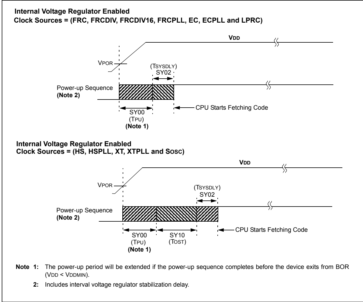
FIGURE 29-4: POWER-ON RESET TIMING CHARACTERISTICS
