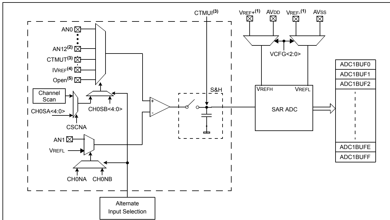
FIGURE 21-1: ADC1 MODULE BLOCK DIAGRAM
