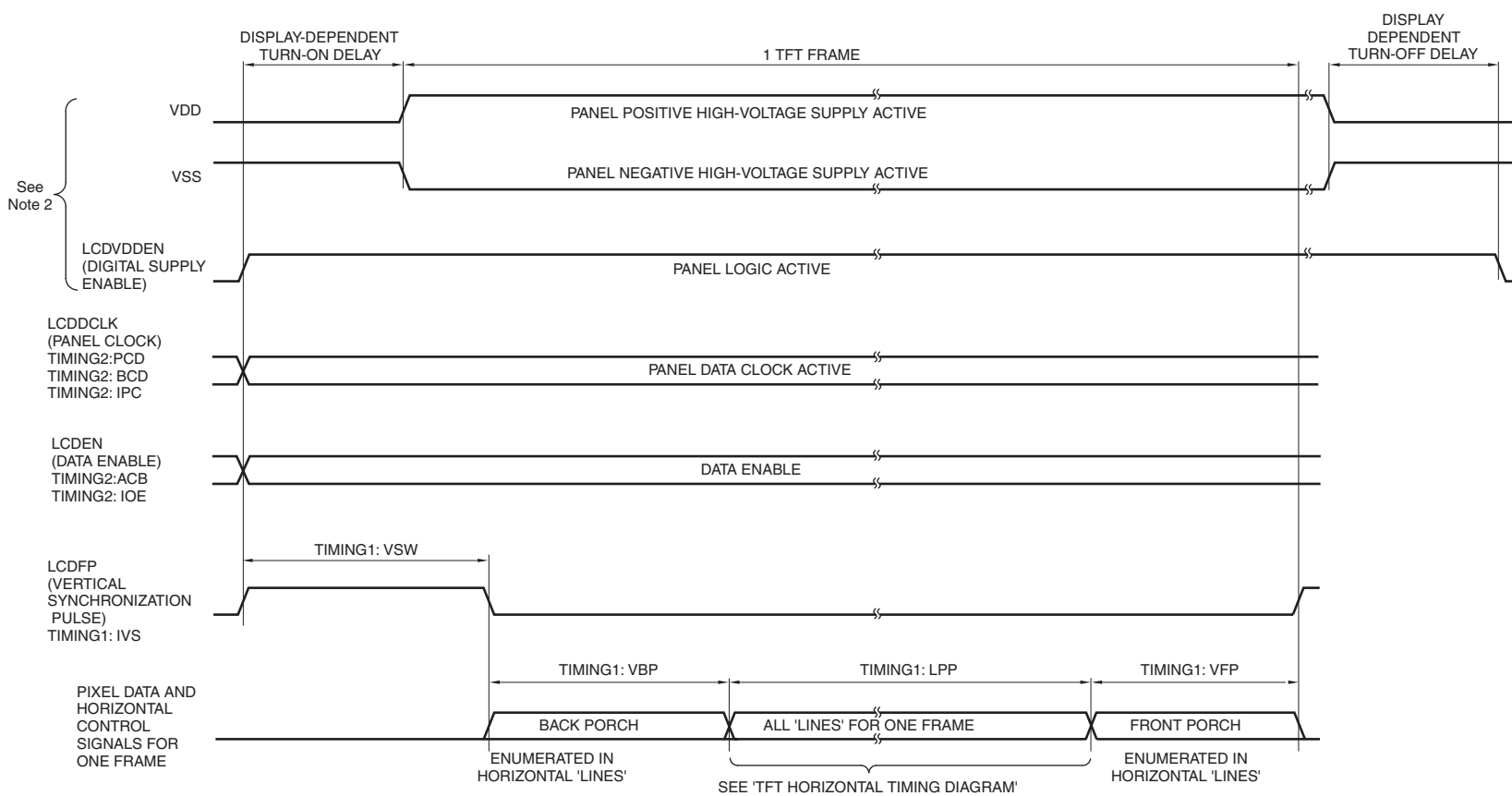
Figure 31. TFT Vertical Timing
