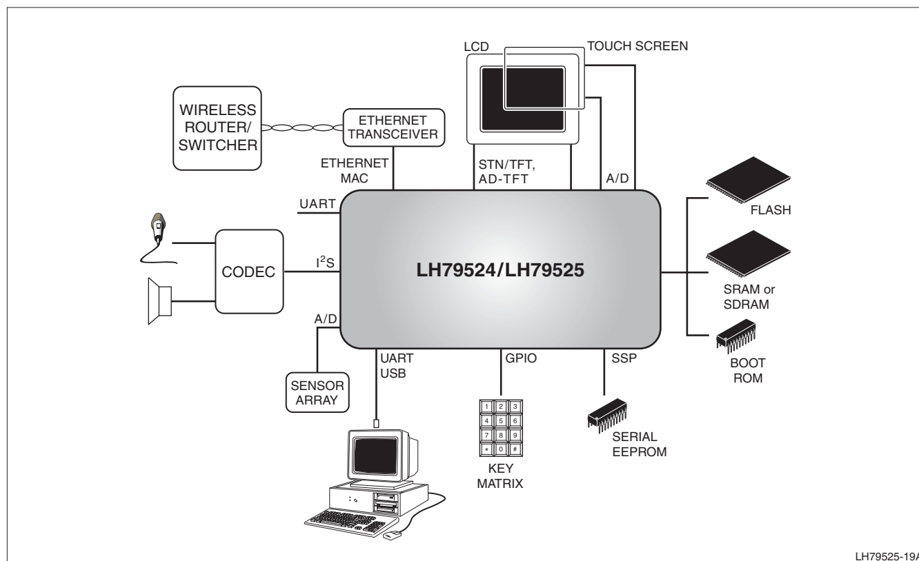
Figure 4. LH79524/LH79525 Application Diagram Example
