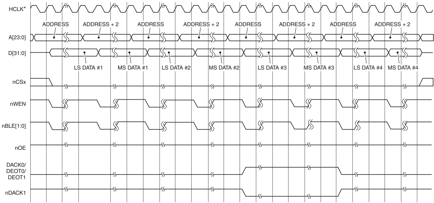
Figure 27. Write, Memory-to-Peripheral: Burst Size = 4; Destination Width > External Access Width
